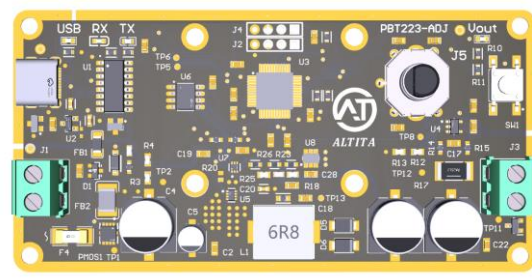
Figure 24 PBT223-ADJ
