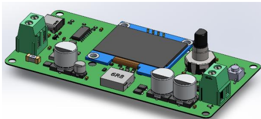
Figure 28 PBT223-ADJ
