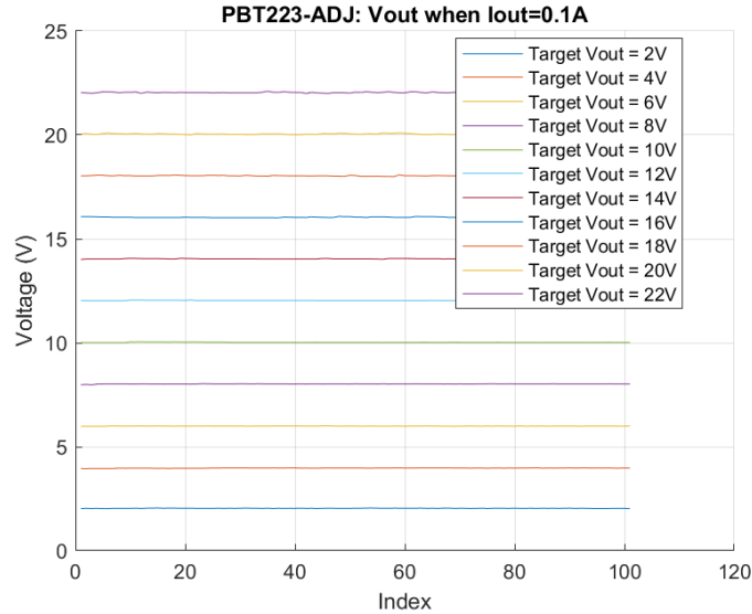
Figure 6 恒电压 CV 模式: I_{out}=0.1\text{A}
