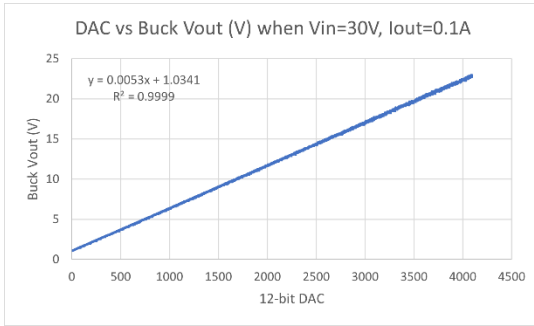
Figure 3 DAC vs Vout when V_{in}=30V , I_{out}=0.1A
