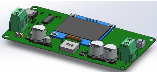
Figure 27 PBT223-FIXED
