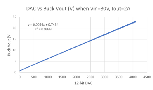
Figure 5 DAC vs Vout when V_{in}=30V , I_{out}=2A
